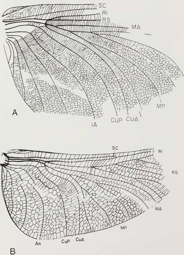
Figure 17A. Moravia grandis , n.sp. Drawing of holotype. Lettering as in figure 12. Permian of Oklahoma.
